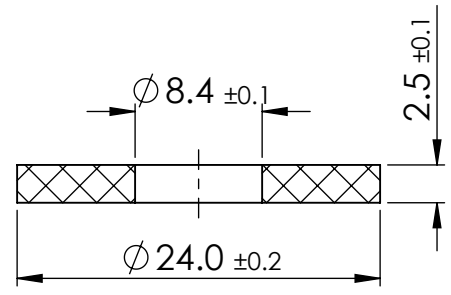
SECTION X-X
